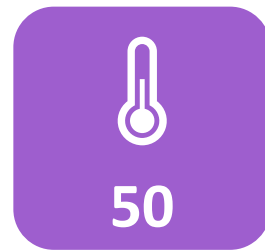
Climate Change
