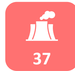
Pollution
